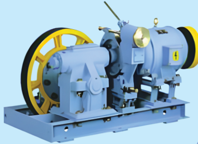
STANDARD TRACTION MACHINE
